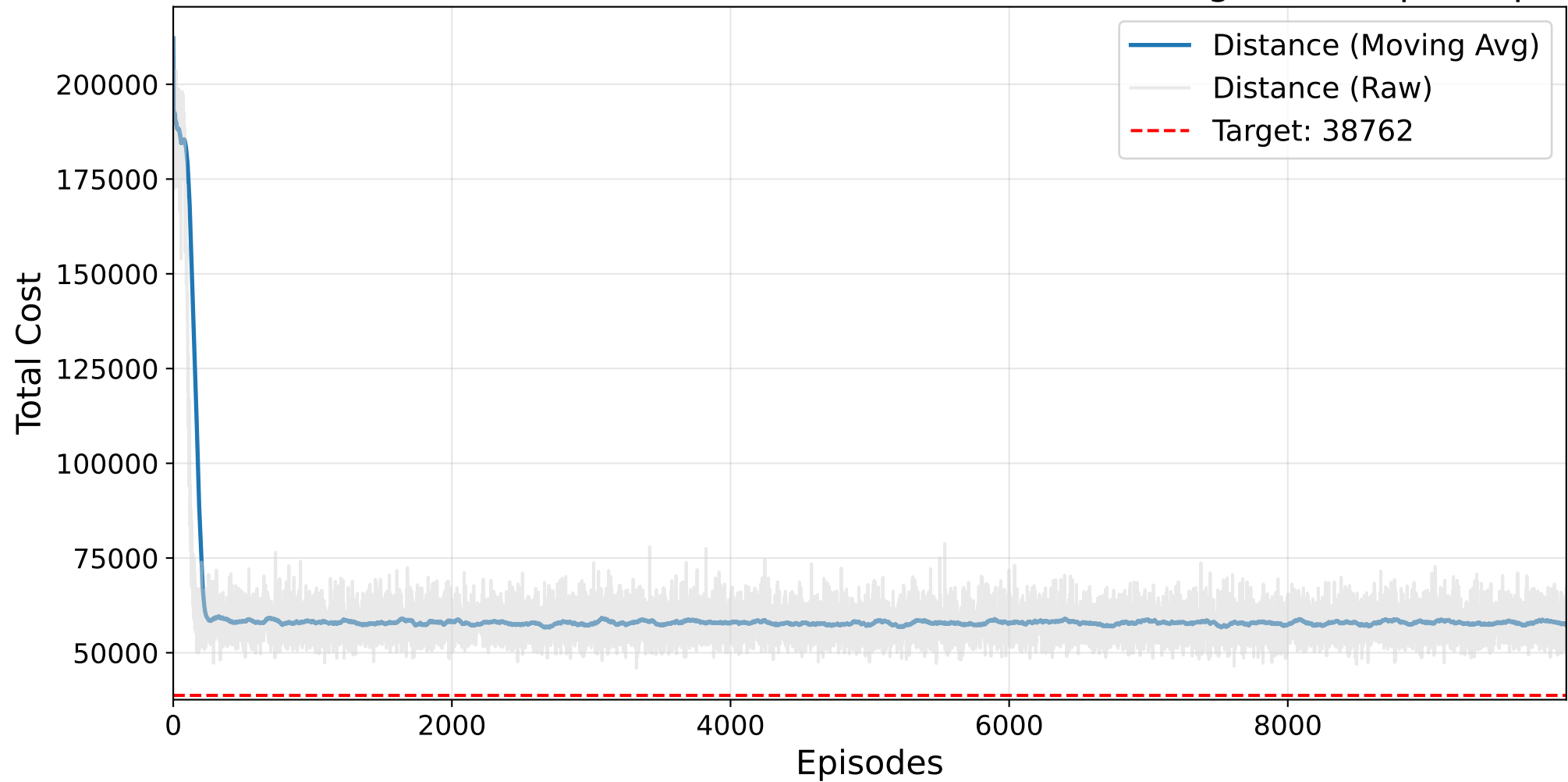
Final GAUSSIAN PROCESS Masked AutoRL-SOP Training - kro124p.1.sop
